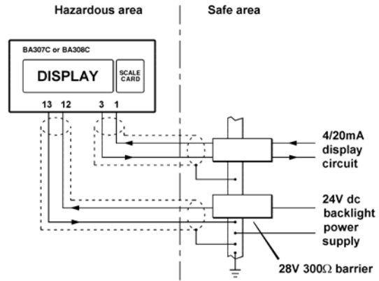
Fig 10 Backlight power supply
