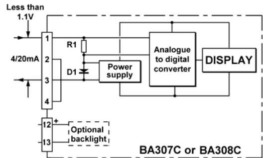
Fig 1 Simplified block diagram of BA307C and BA308C
