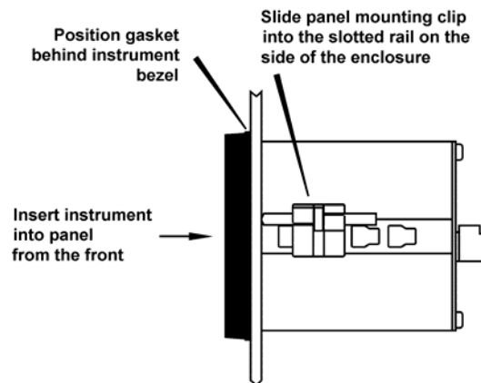
Fig 5 Fitting panel mounting clips
