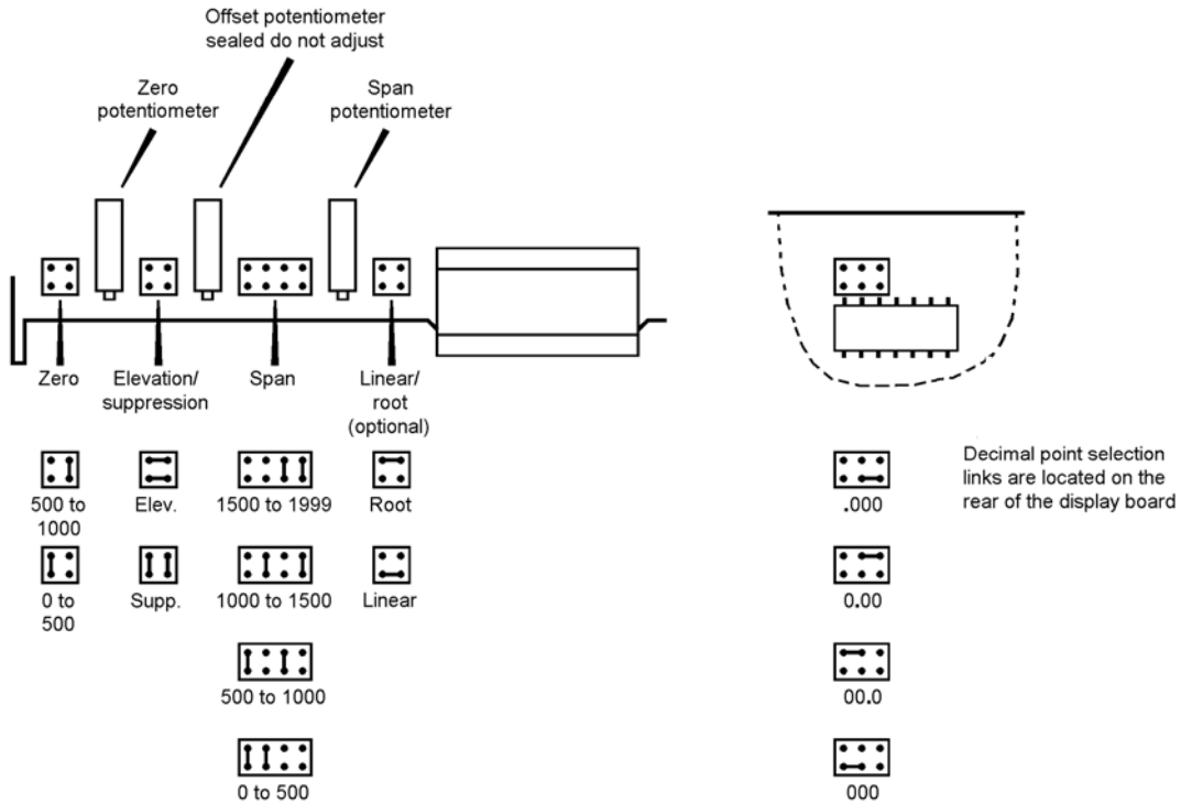
Fig 7 Position of plug-in calibration links and potentiometers
