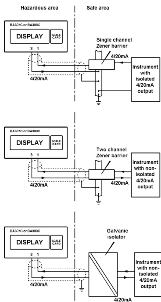
Fig 3 Alternative circuits for remote indication in hazardous area
