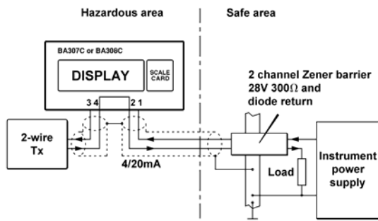
Fig 2 BA307C or BA308C in a transmitter loop
